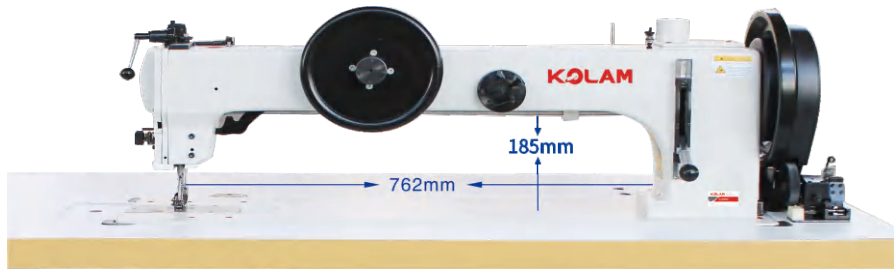
KL-204-762 单针长臂综合送料厚料缝纫机 Single-needle long-arm comprehensive feeding thick material sewing machine
