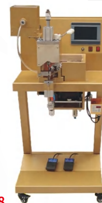
KL-198 全自动四爪底扣珍珠钉扣机 Automatic Four Claws Nail Base Button Plastic Pearl Attaching Machine(single head)
